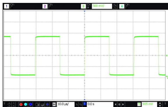
Figure 15. LVCMOS Output Waveform ( V_{Swing} = 1.8\text{V} , SiT1534AI-J4-DCC-32.768)
