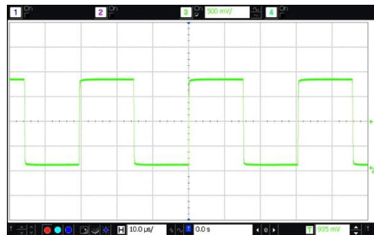
Figure 7. LVCMOS Waveform (V DD = 1.8V) into 15 pF Load
