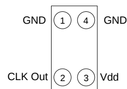
Figure 2. Pin Assignments (CSP)
