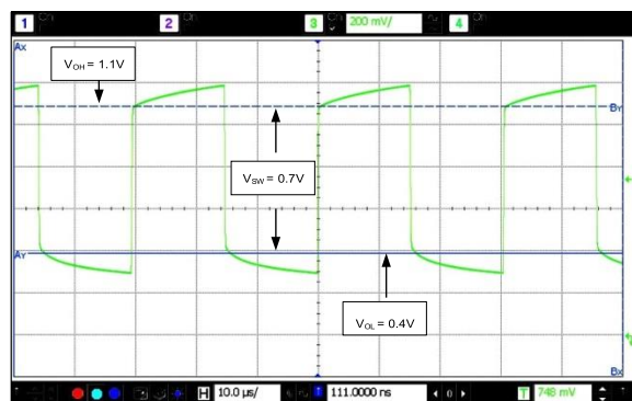
Figure 6. SiT1534AI-J4-D14-32.768 Output Waveform (10 pF load)
