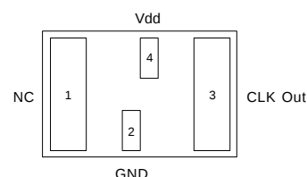
Figure 1. Pin Assignments (SMD)
