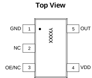
Figure 1. Pin Assignments
