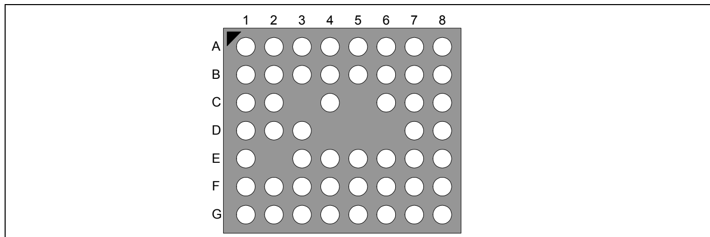
Figure 8. 50-Ball 4.5 x 4 x 0.6 mm (FPBGA) Array
