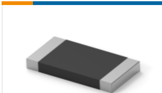
TE Part #6-2176422-4 TLRP 2512 3.0W R039 1% 50PPM 4K RL
