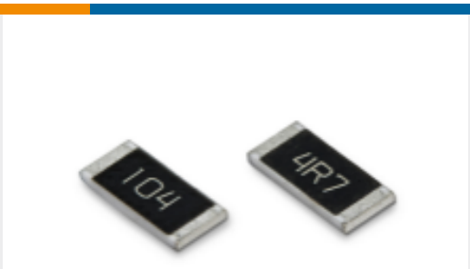
TE Part #2-1879207-1 RN 0603 324K 0.1% 10PPM 5K RL
