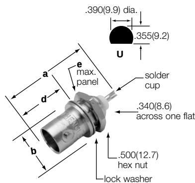
75Ω BNC Receptacles (J) Front Mount 31-221-75RFX 31-70018 31-71004
