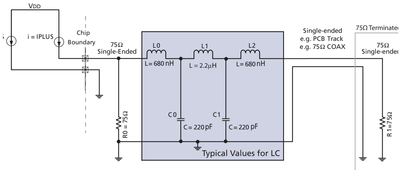
Figure 21: Single-Ended Termination
