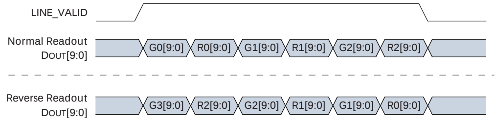
Figure 16: Six Pixels in Normal and Column Mirror Readout Modes
