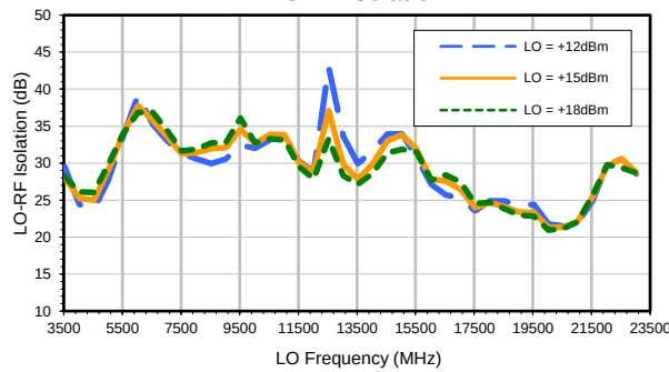
LO-RF Isolation
