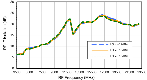
RF-IF Isolation
