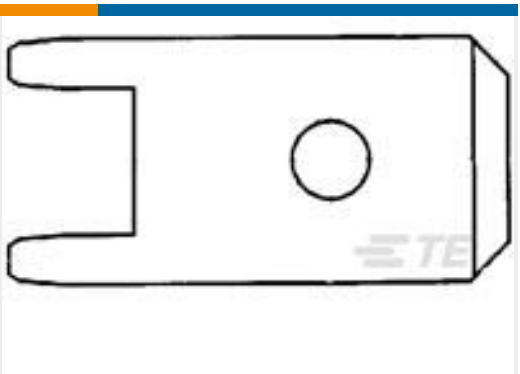
TE Part #170267-1 250 FASTON,PCB TAB,TCBR
