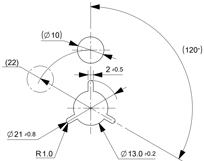
DETAIL "Z"
