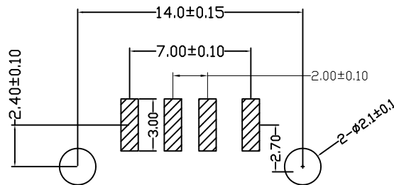
PCB LAYOUT
