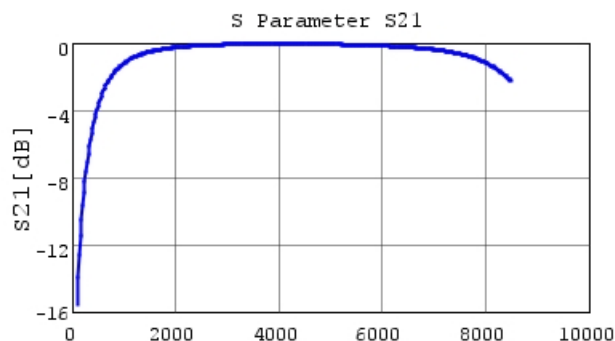
GRM1885C2A2R7CA01 S21 DCOV, 25degC
