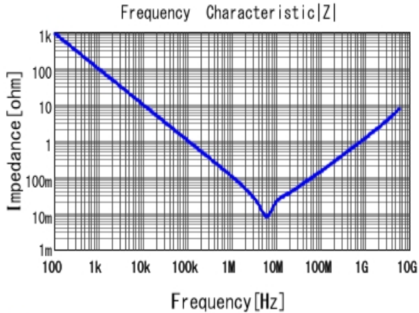
■ GRM155Z71A225ME43 |Z| DC0V, 25degC
