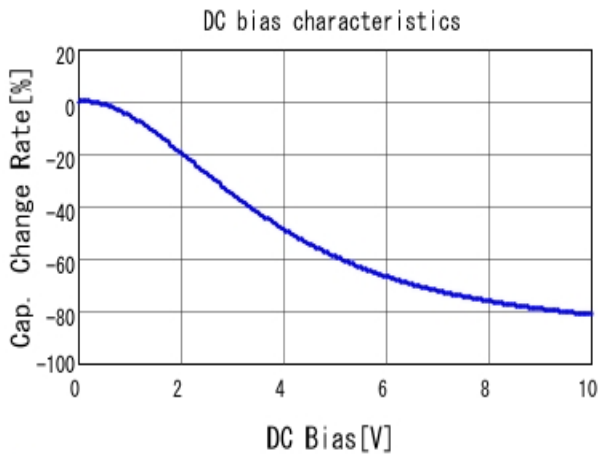
■ GRM155Z71A225ME43 C-DC bias capchange, 25.0degC, AC1V
