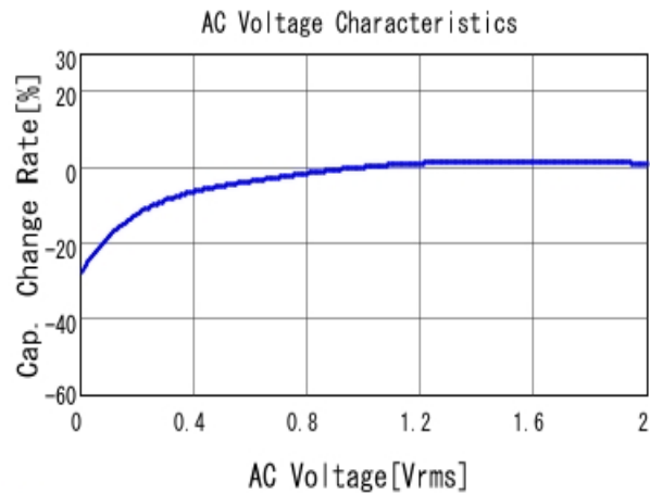
■ GRM155Z71A225ME43 C-AC Voltage capchange, DC0V, 25.0d
