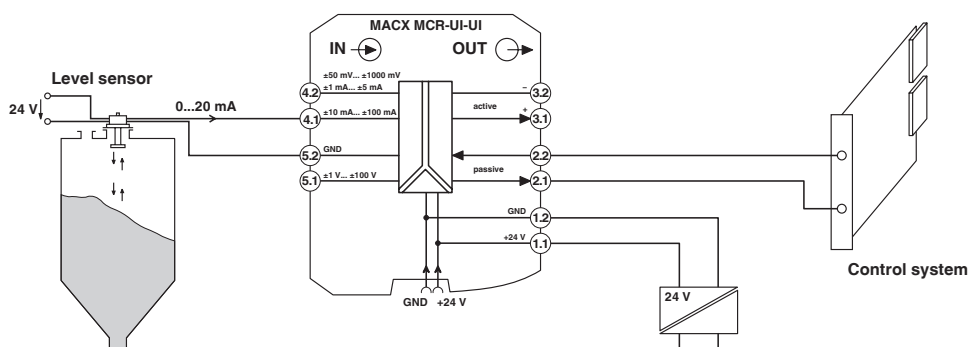
Application drawing
