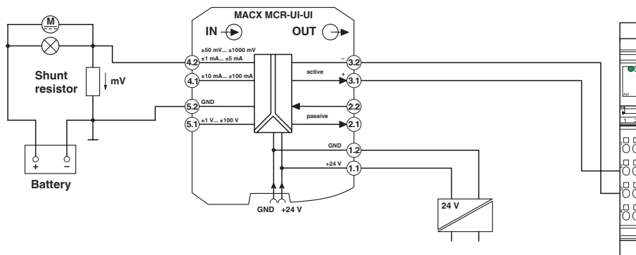
Application drawing
