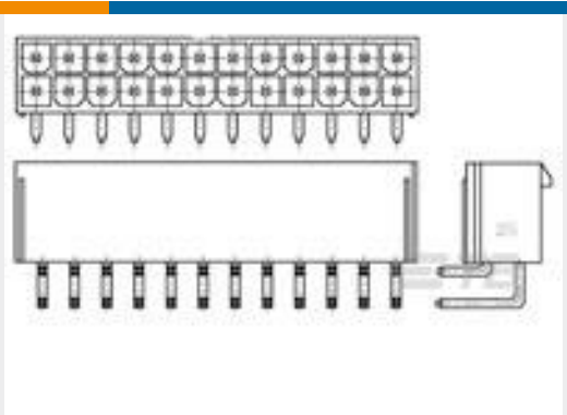
TE Part #1586042-4 4P VAL-U-LOK R/A HDR V0
