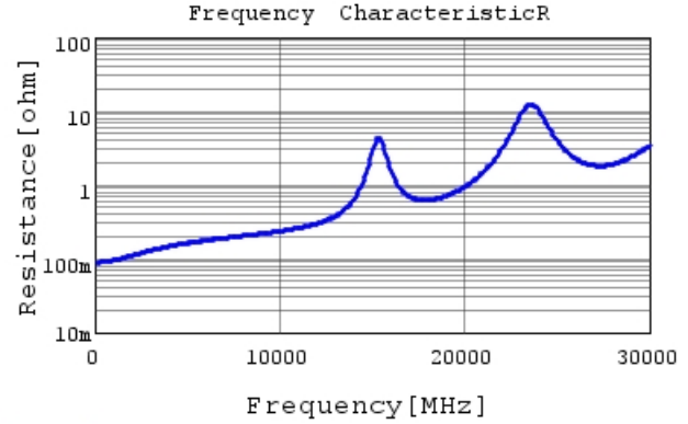
GJM0335C2A4R4BB01 R DC0V, 25degC
