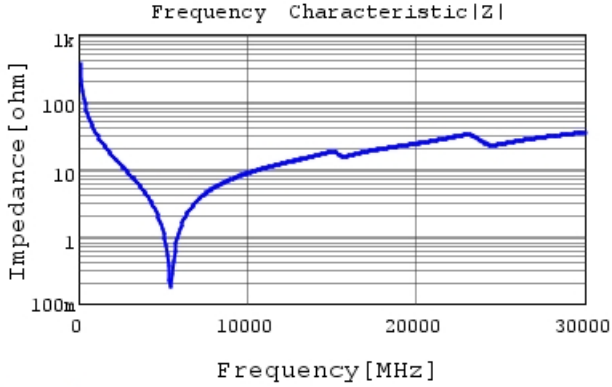
GJM0335C2A4R4BB01 |Z| DC0V, 25degC
