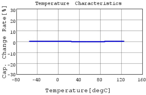
GJM0335C2A4R4BB01 C-Temp. capchange, DCOV, 1
