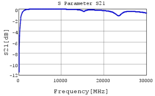
GJM0335C2A4R4BB01 S21 DCOV, 25degC
