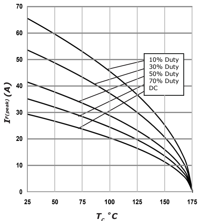
Figure 3. Current Derating
