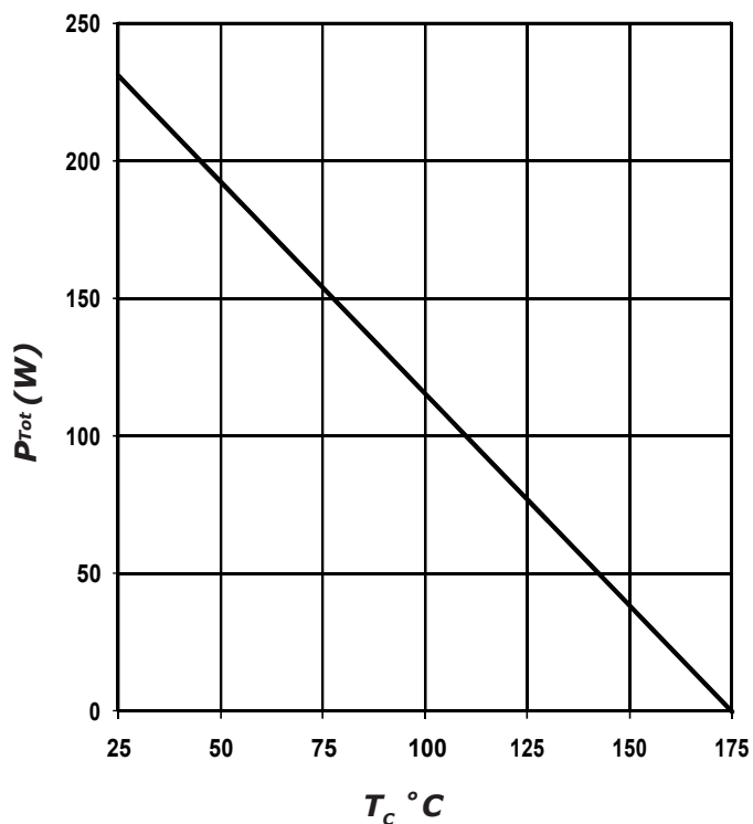
Figure 4. Power Derating
