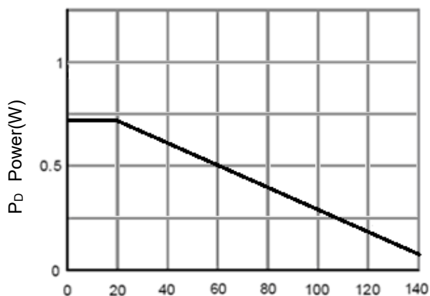
Figure 3 Power Dissipation
