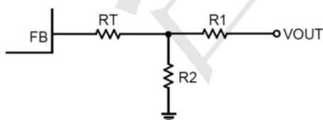
Figure 3: T-Type Network
