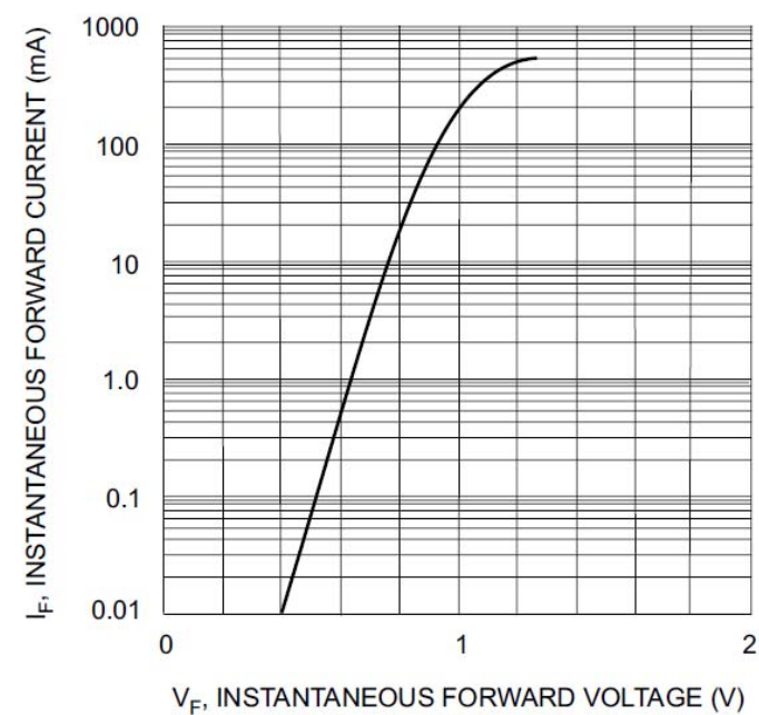
Fig. 1 Forward Characteristics
