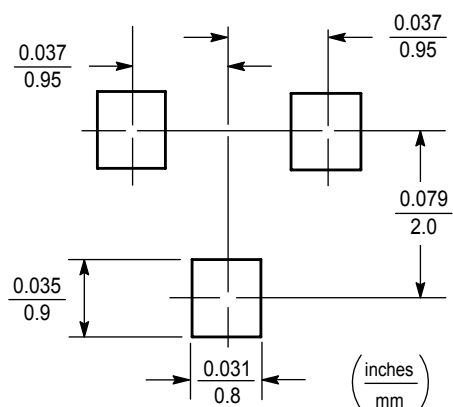
Soldering Footprint:
