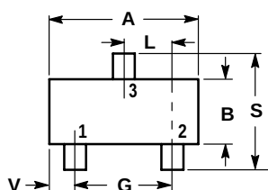
Dimension Outline:
