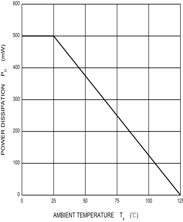
Power Derating Curve
