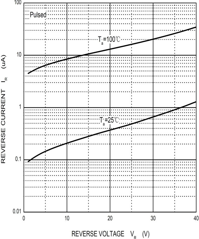
Reverse Characteristics
