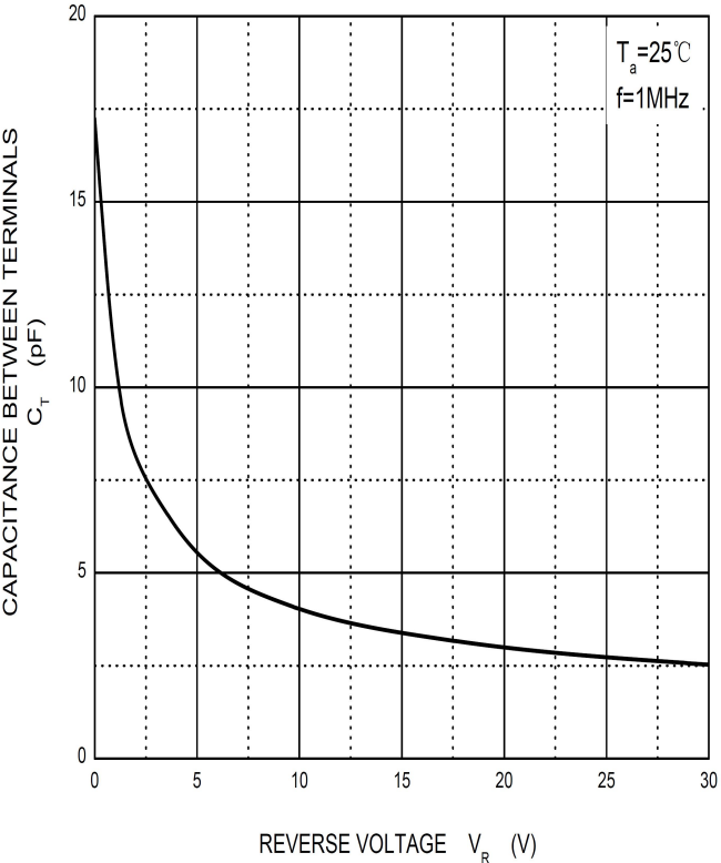
Capacitance Characteristics
