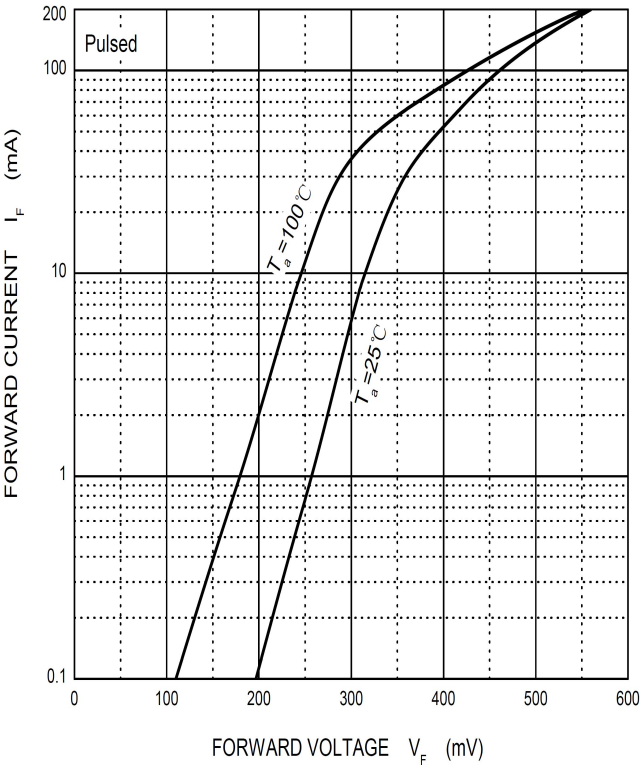
Forward Characteristics
