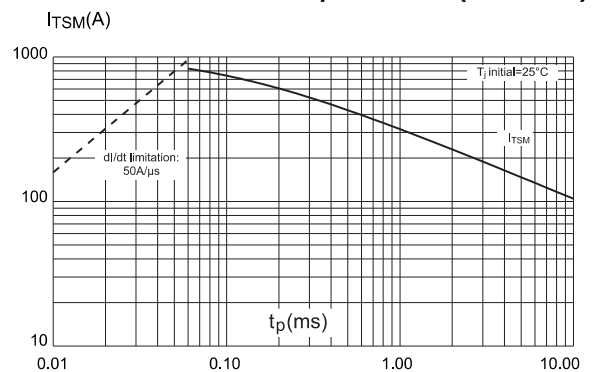
Figure 6: Non repetitive surge peak on-state current versus sinusoidal pulse width ( t_p < 10 \text{ ms} )
