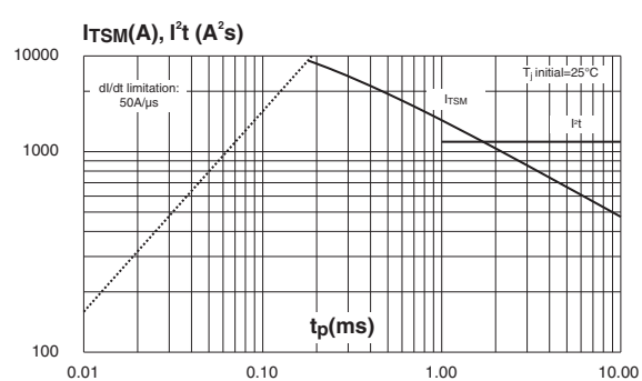
Figure 6: Non-repetitive surge peak on-state current for a sinusoidal pulse with width t_p < 10\text{ ms} and corresponding value of I^2t
