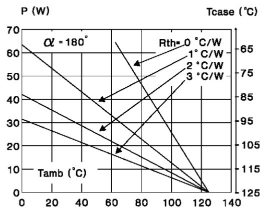
Fig.4 : Correlation between maximum average power dissipation and maximum allowable temperatures ( T_{amb} and T_{case} ) for different thermal resistances heatsink + contact (BTW 69 N).
