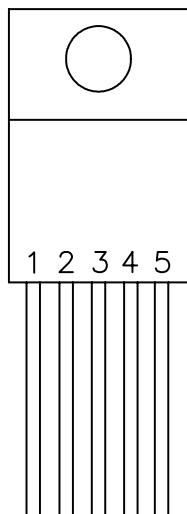
TO-220-5
