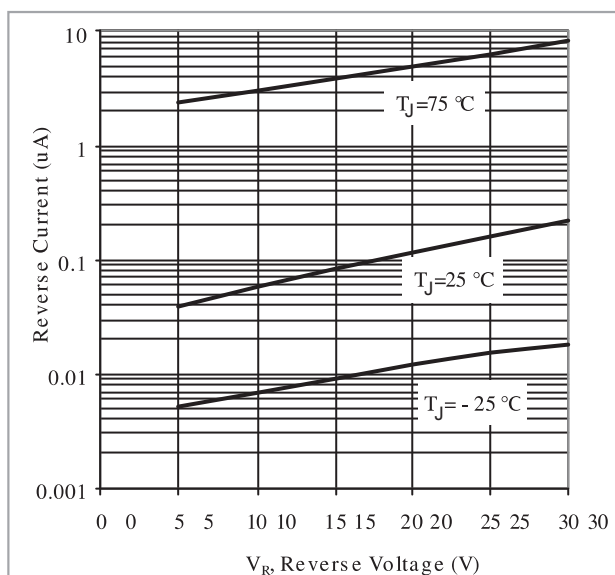
FIG. 1-Typical Reverse Leakage
