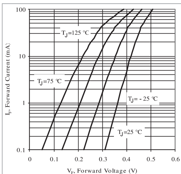
FIG. 2-Typical Forward Voltage
