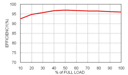
DOS10-05T, Vout=3.3V Efficiency vs. Output Load
