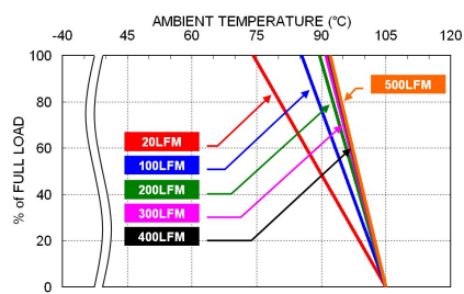
EDL03-24S05W Derating Curve
