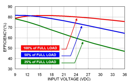
EDL03-24S05W Efficiency vs. Input Voltage
