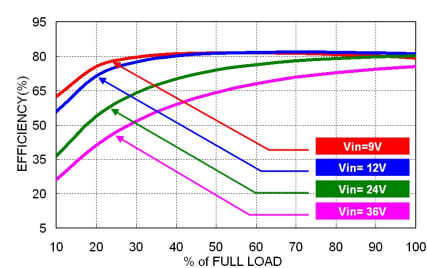
EDL03-24S05W Efficiency vs. Output Load
