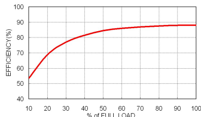
FEC15-48S05W Efficiency vs. Output Load
