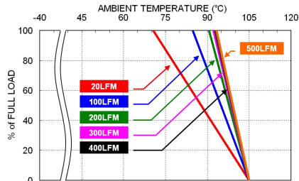
FED40-48S05W Derating Curve
