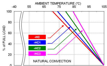
FED40-48S05W Derating Curve With Heat-sink
