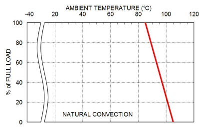
FKC05-48S05-M1 Derating Curve
