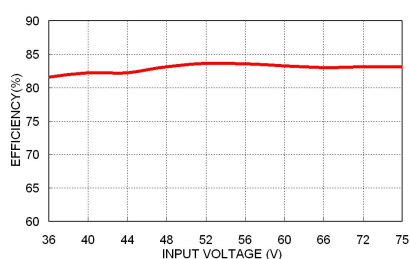
FKC08-48S05 Efficiency vs. Input Voltage
