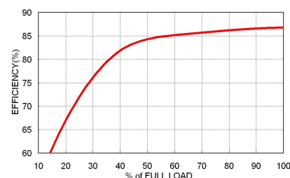
FKC12-48S05 Efficiency vs. Output Load
