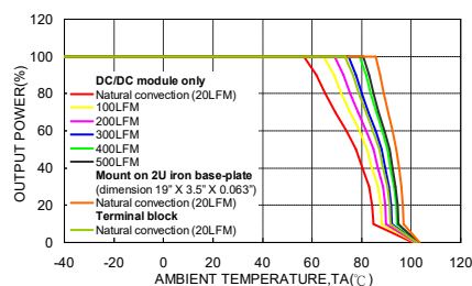
HAE100-48S05W Derating Curve (See Thermal Considerations)
