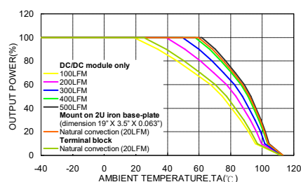
HAE200-48S05W Derating Curve (See Thermal Considerations)
