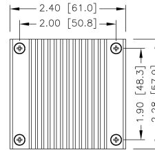
HAE75-□□S□□W - HS1 7G-0022A-F
