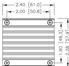
HAE75-□□S□□W - HS4 7GA0127P01-F
