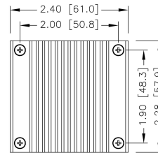
HAE75-□□S□□W - HS3 7G-0024A-F
