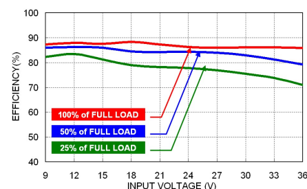
MPM15-24S05W Efficiency vs. Input Voltage
