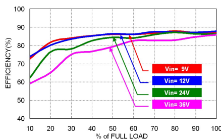
MPM15-24S05W Efficiency vs. Output Load
