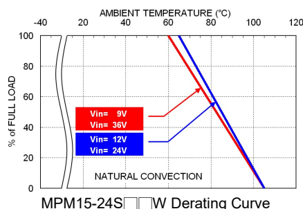
MPM15-24S□□W Derating Curve
