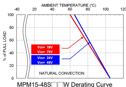
MPM15-48S□□W Derating Curve
