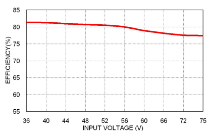
PDL03-48S05 Efficiency vs. Input Voltage
