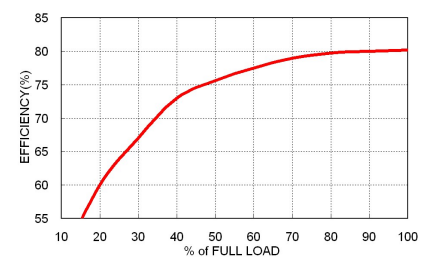
PDL03-48S05 Efficiency vs. Output Load
