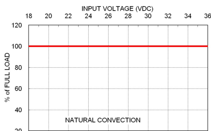
PDL09-24S12M Load Derating v.s. Input Voltage (at T_a = 60^\circ\text{C} )
