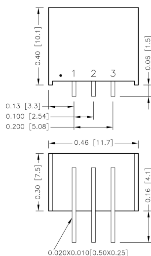
BOTTOM VIEW
