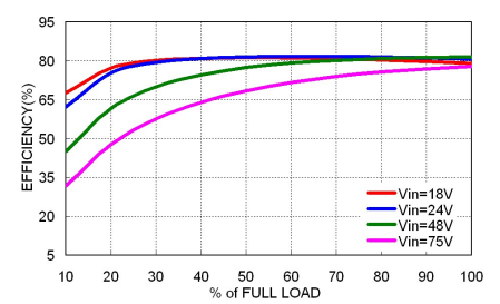
SDS(H)05-48S05W Efficiency vs. Output Current
