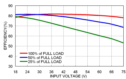
SDS(H)05-48S05W Efficiency vs. Input Voltage
