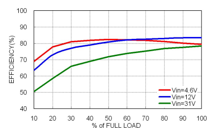
SSR01-12S05 Efficiency VS Output Load
