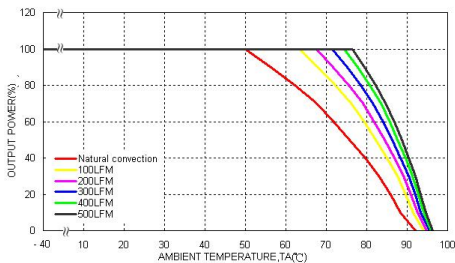
WAF(D)150-48S24W Derating Curve (See Thermal Consideration)
