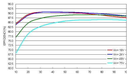
WAF(D)150-48S24W Efficiency vs. Output Load
