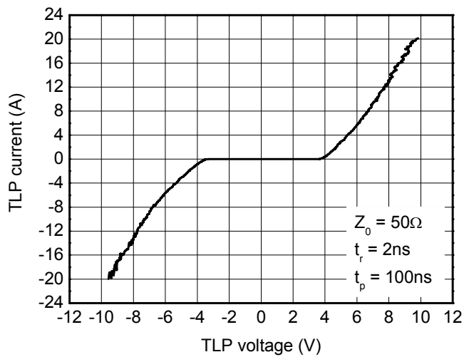
TLP Measurement
