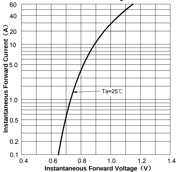
FIG3: Forward Voltage
