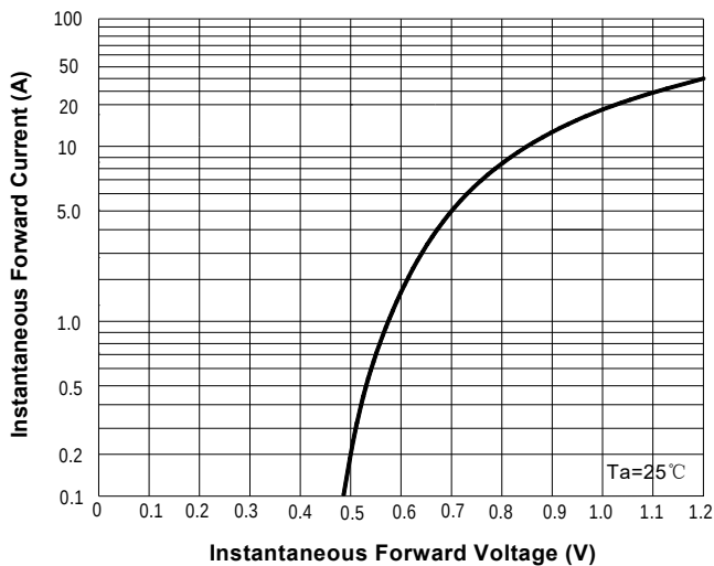
FIG3: Forward Voltage
