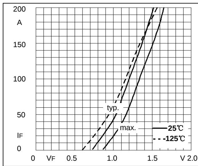
Fig1. Forward Characteristics
