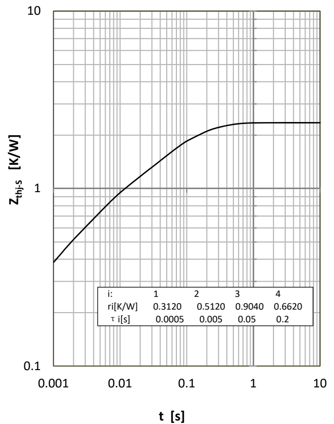
Fig 10. IGBT Transient Thermal Impedance
