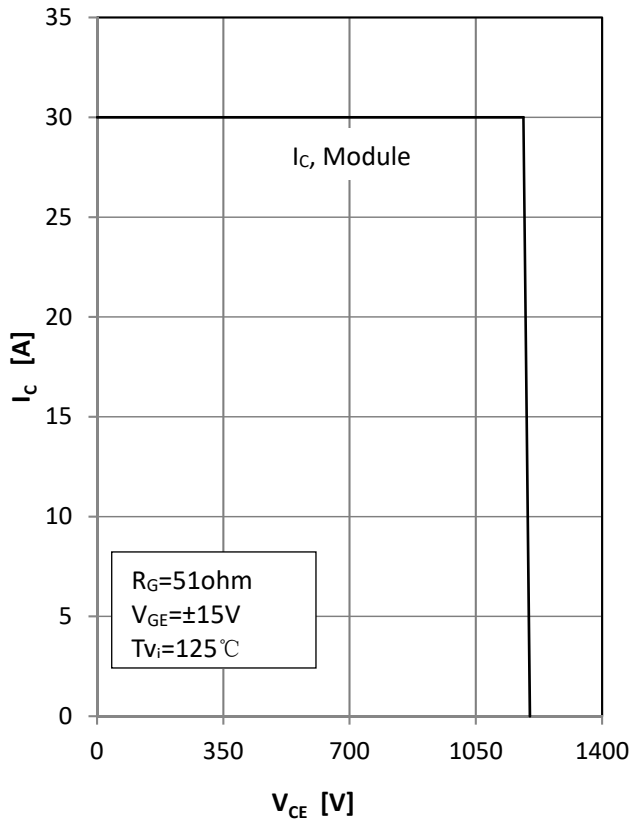
Fig5. RBSOA
