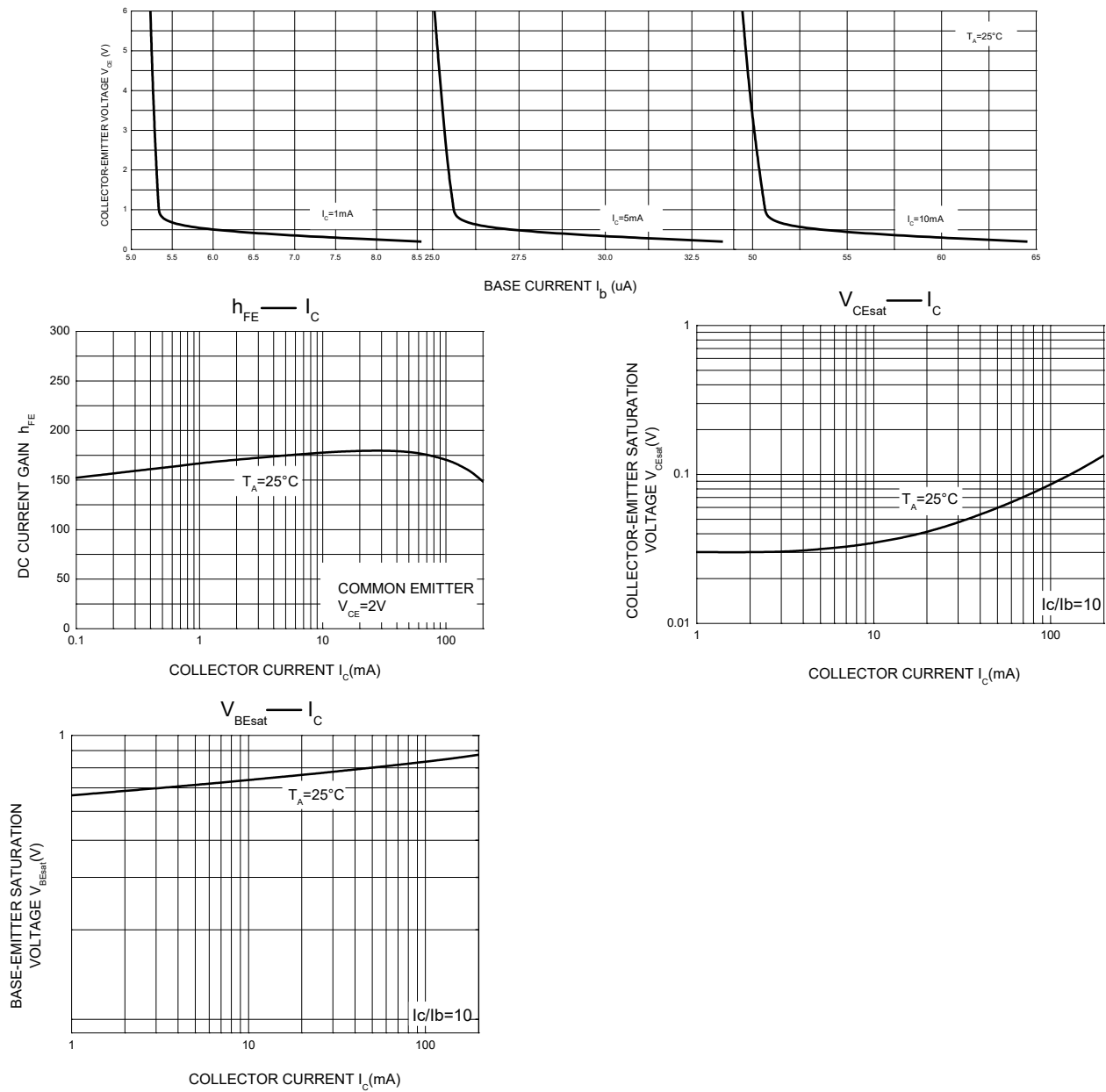
Static Characteristics
